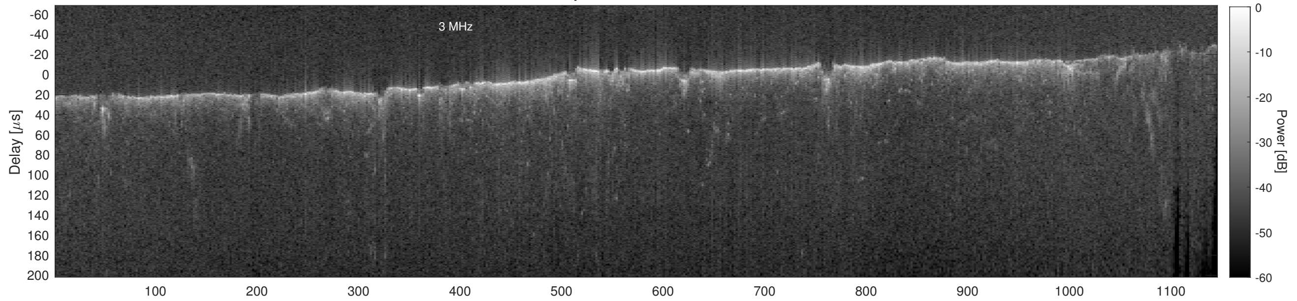
Orbit 11160, Cluttergram
