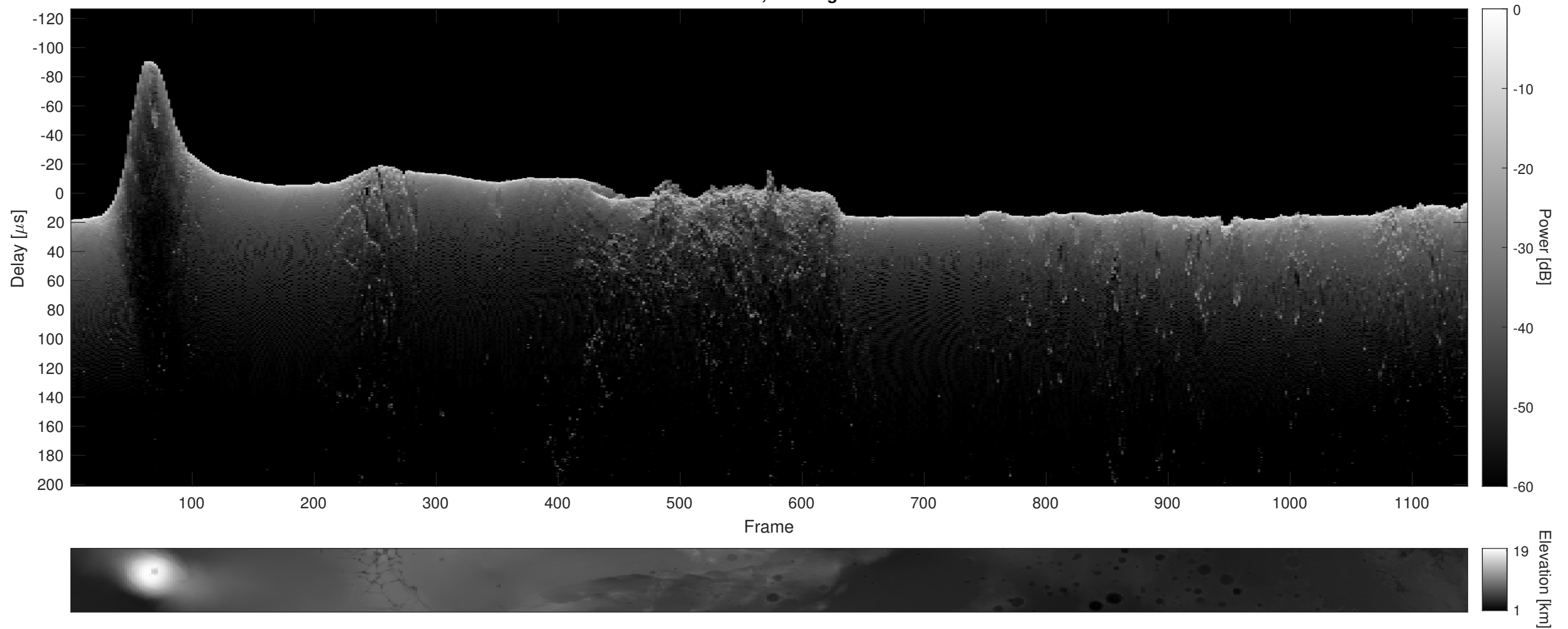
Orbit 11161, Cluttergram
