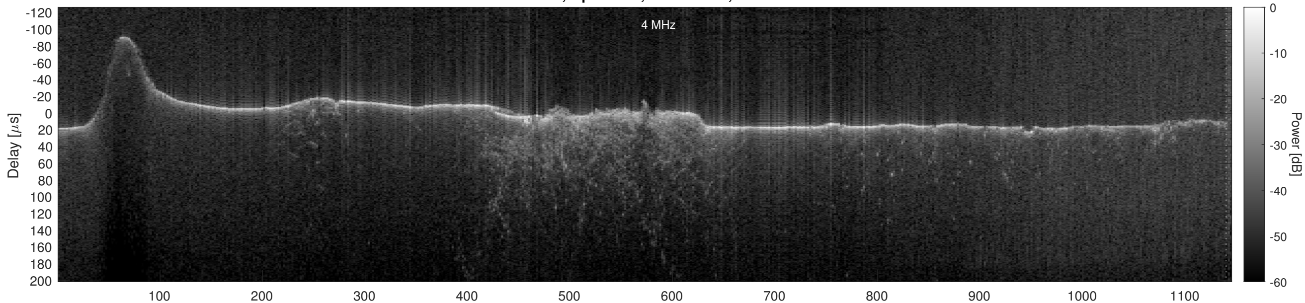
Orbit 11161, Optimized, No Window, Channel 2
