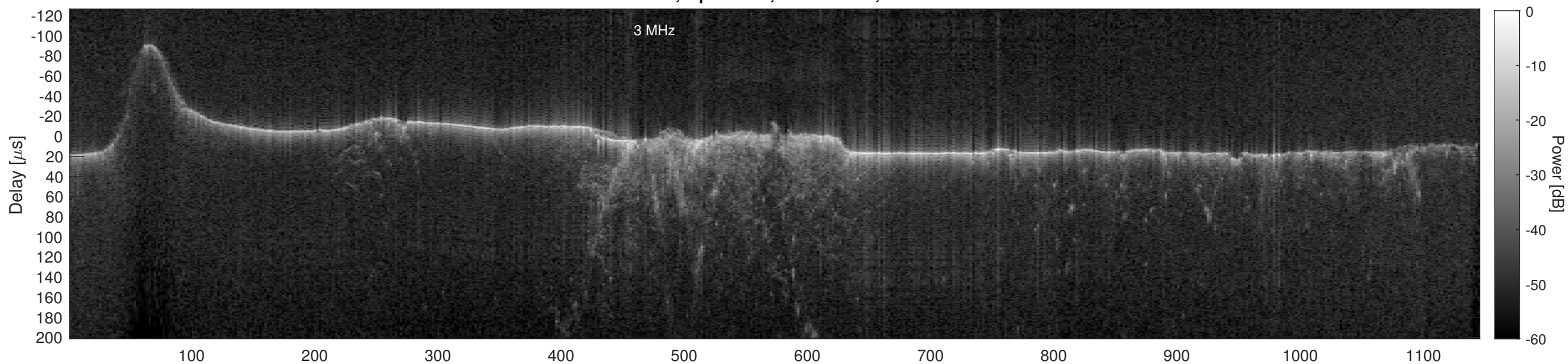
Orbit 11161, Cluttergram
