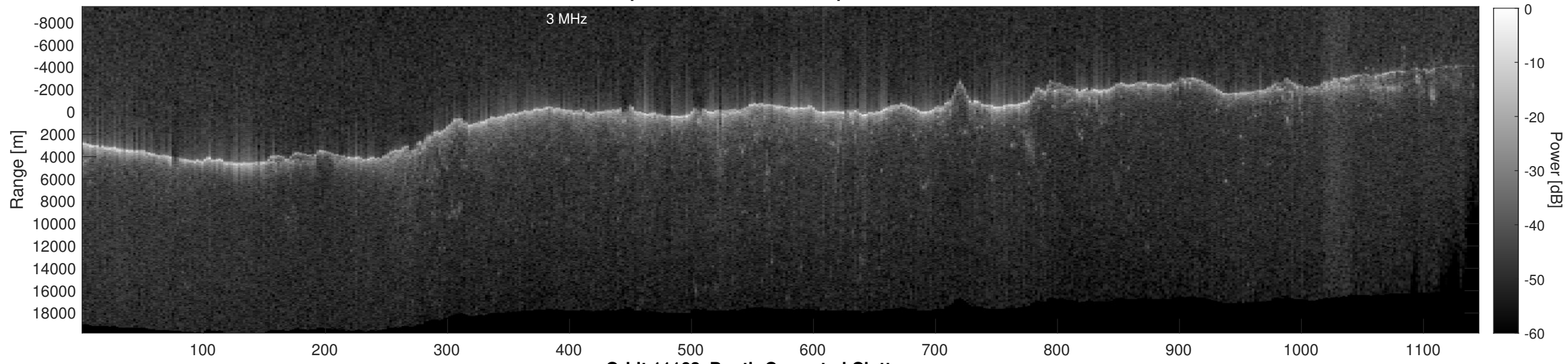
Orbit 11162, Depth-Corrected Cluttergram
