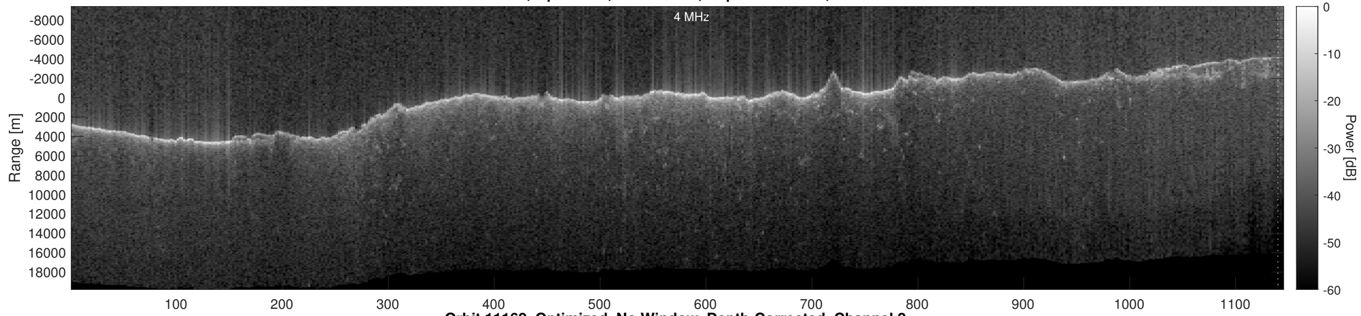
Orbit 11162, Optimized, No Window, Depth-Corrected, Channel 2
