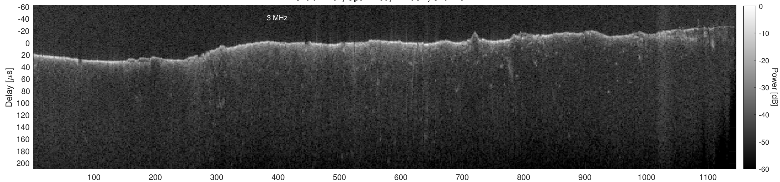
Orbit 11162, Cluttergram
