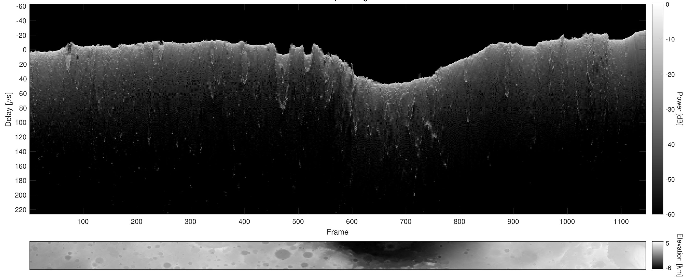
Orbit 11163, Cluttergram
