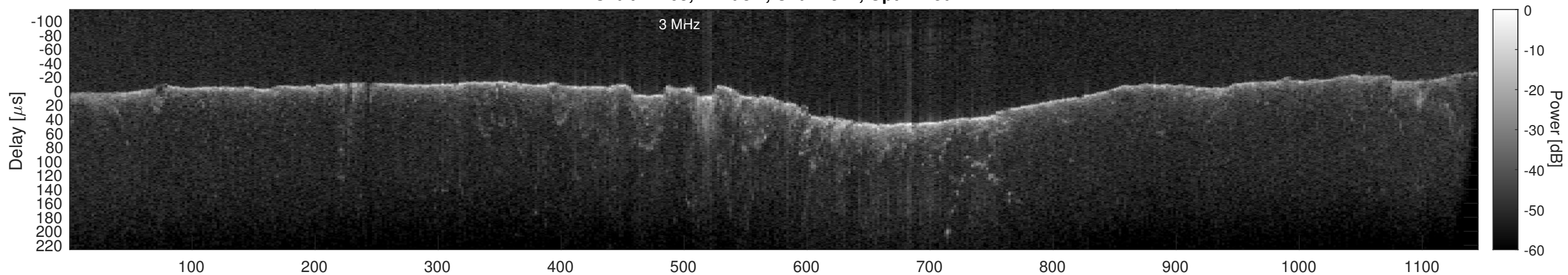
Orbit 11163, Cluttergram
