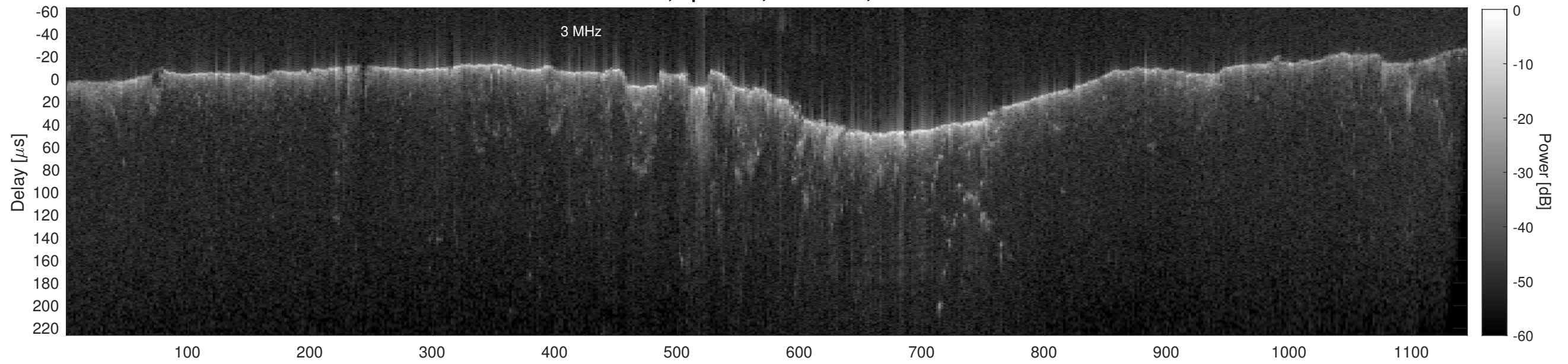
Orbit 11163, Cluttergram
