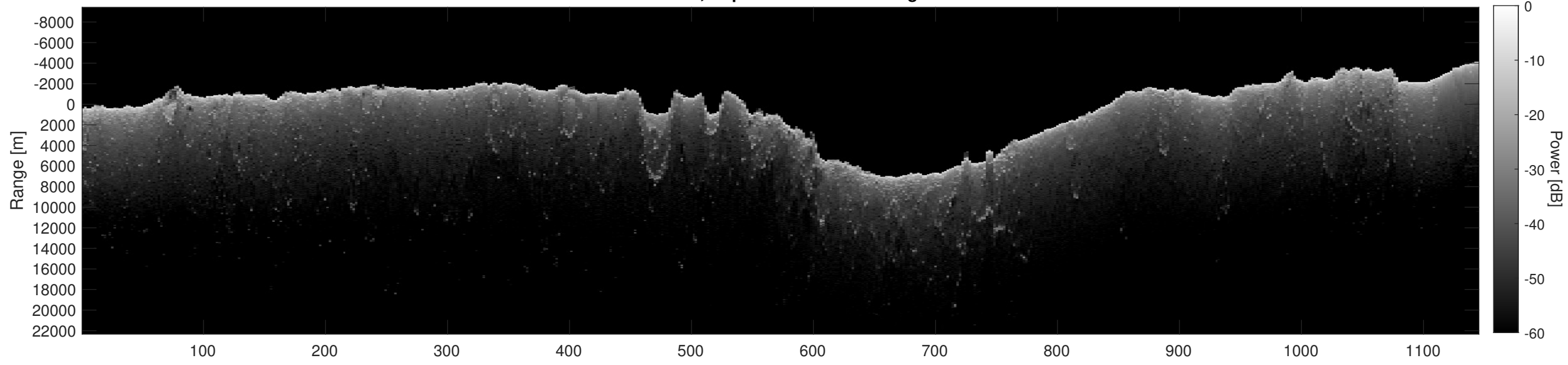
Orbit 11163, Depth-Corrected Cluttergram
