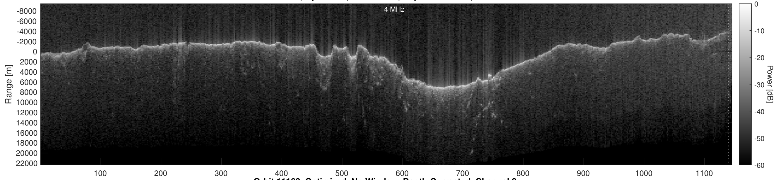
Orbit 11163, Optimized, No Window, Depth-Corrected, Channel 2
