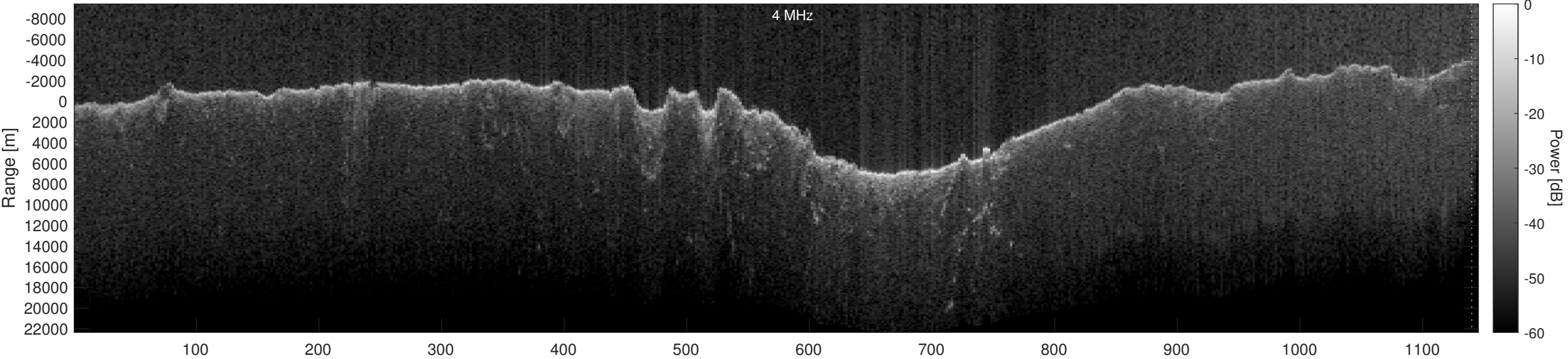
Orbit 11163, Optimized, Window, Depth-Corrected, Channel 2
