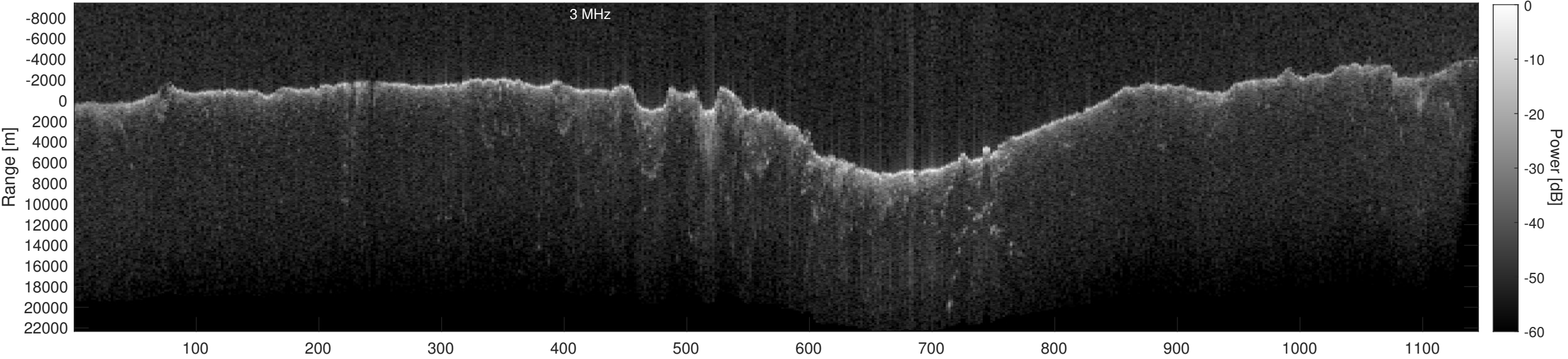
Orbit 11163, Depth-Corrected Cluttergram
