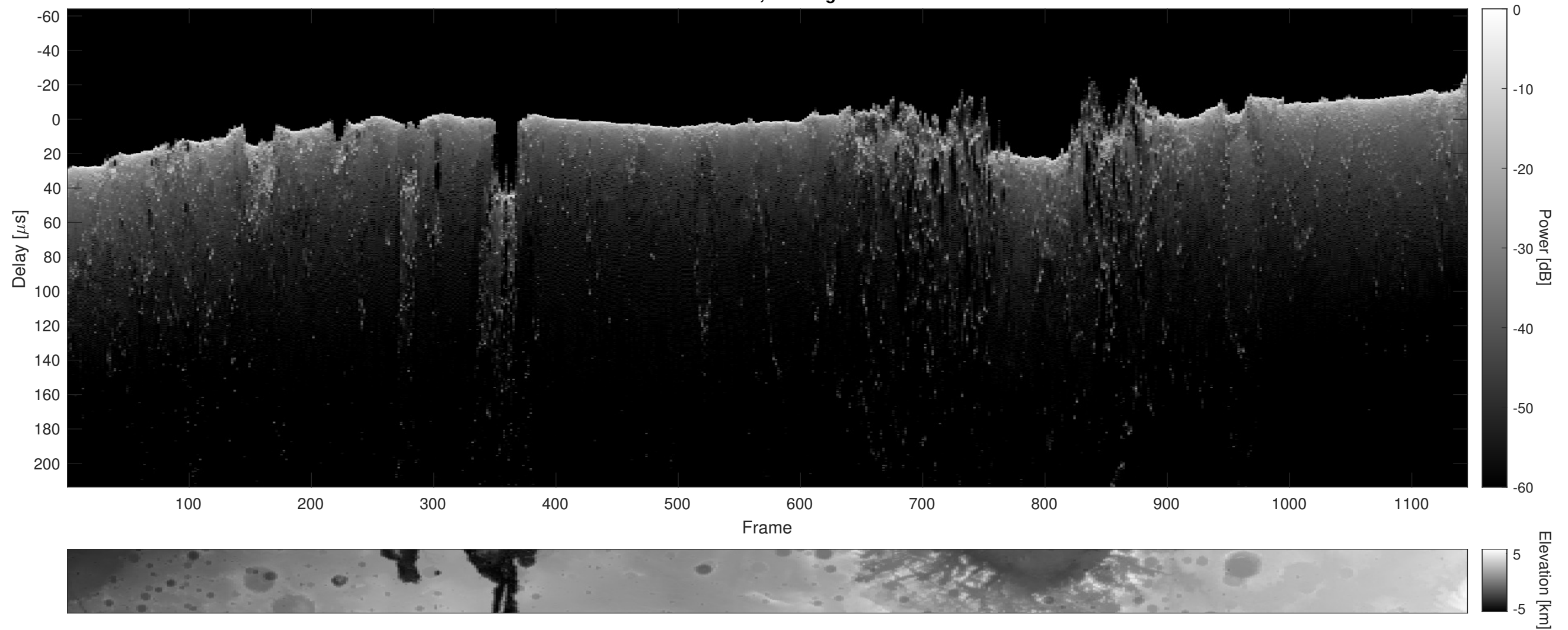
Orbit 11164, Cluttergram
