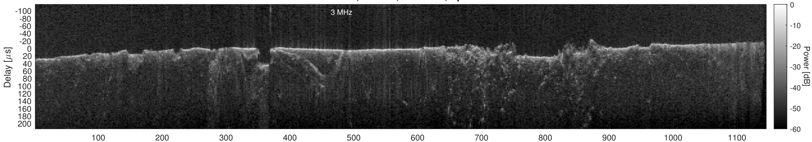
Orbit 11164, Cluttergram
