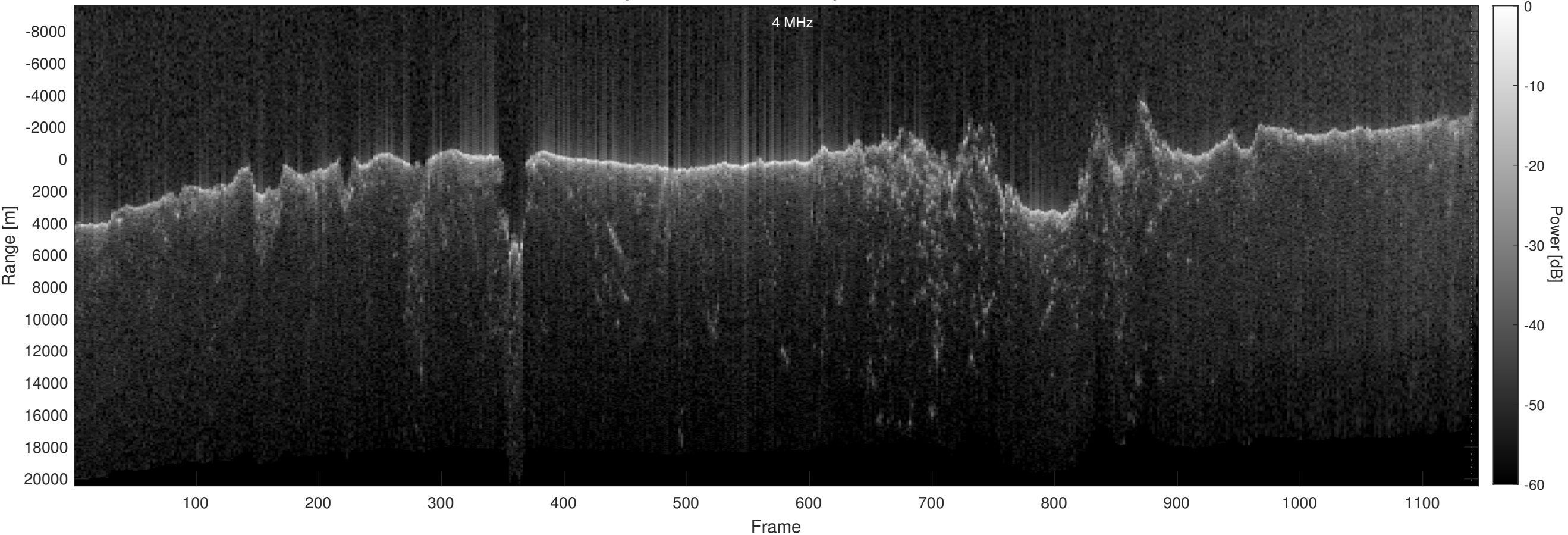
Orbit 11164, Optimized, No Window, Depth-Corrected, Channel 2
