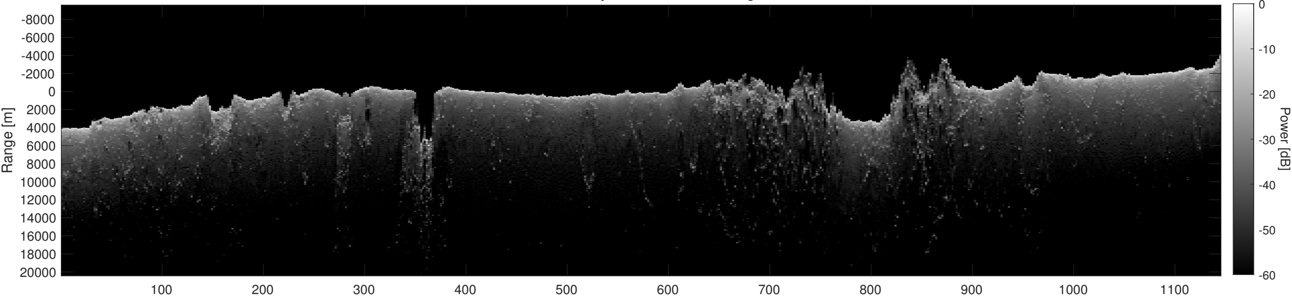
Orbit 11164, Depth-Corrected Cluttergram
