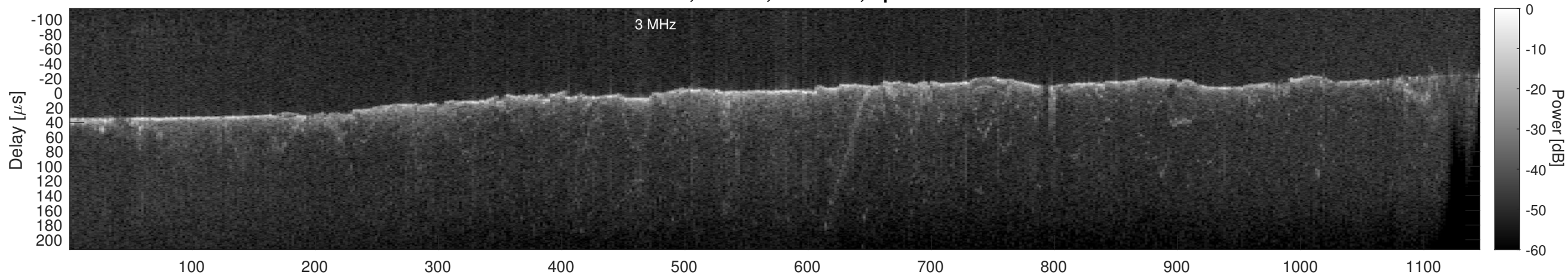
Orbit 11165, Cluttergram
