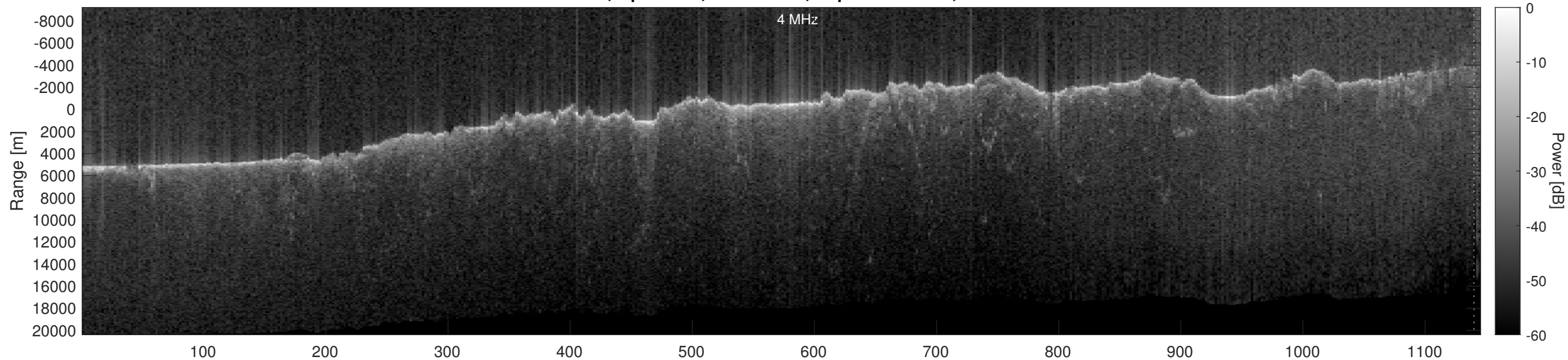
Orbit 11165, Optimized, No Window, Depth-Corrected, Channel 2
