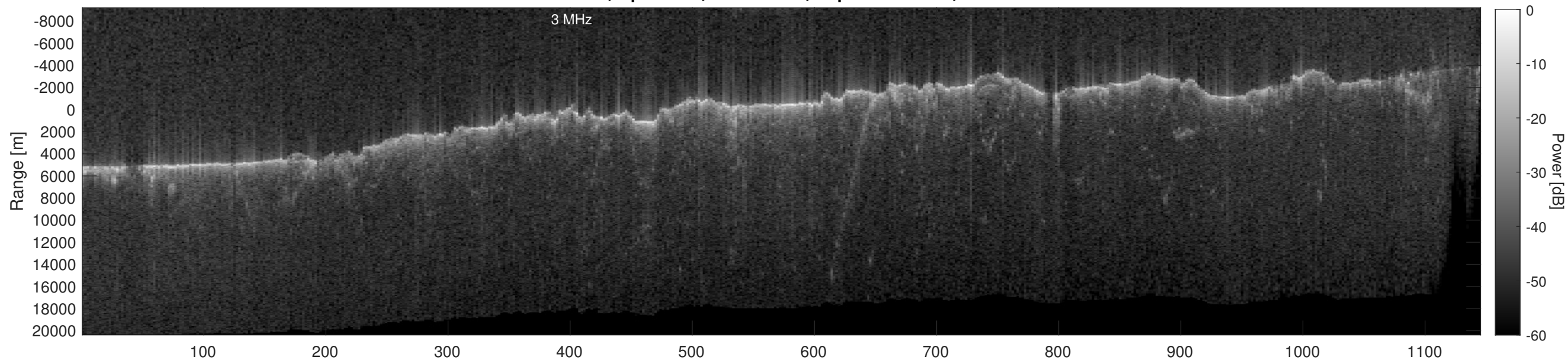
Orbit 11165, Depth-Corrected Cluttergram
