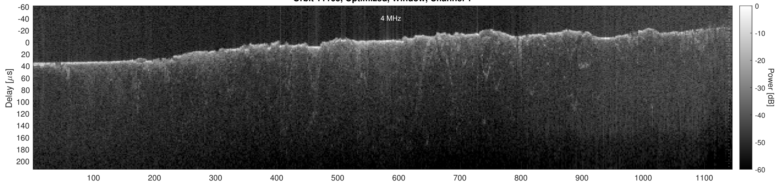
Orbit 11165, Optimized, Window, Channel 2
