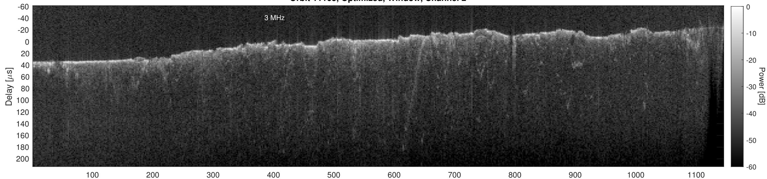
Orbit 11165, Cluttergram
