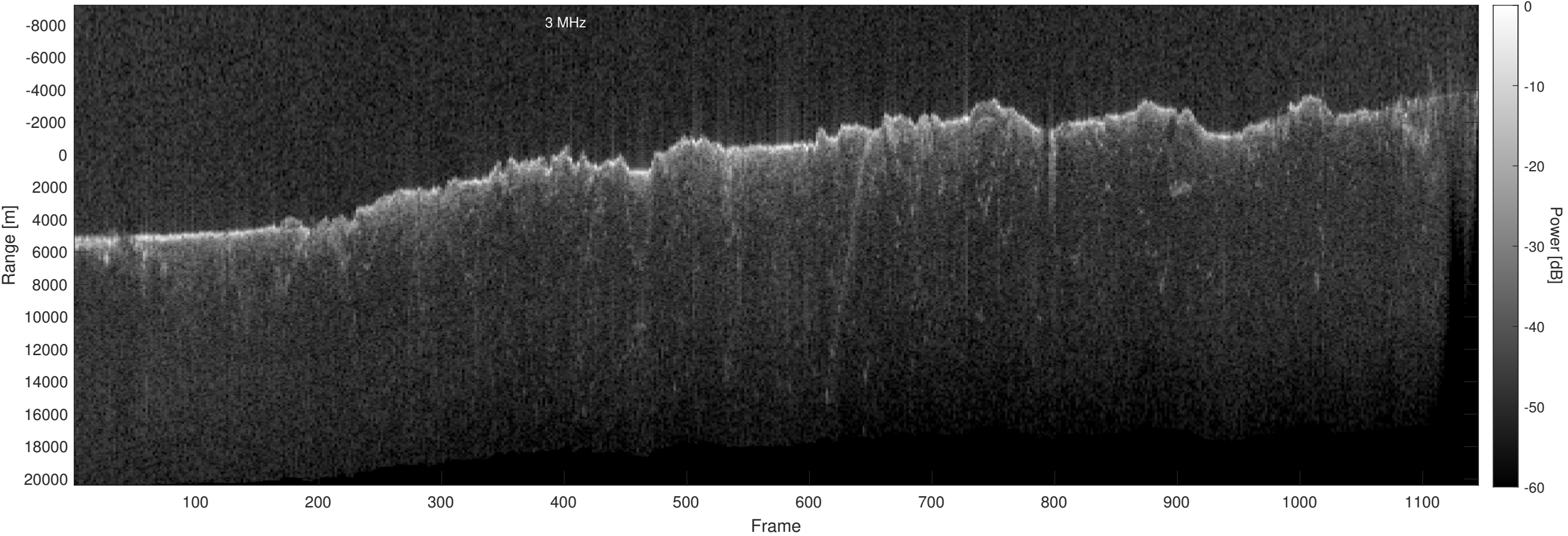
Orbit 11165, Optimized, Window, Depth-Corrected, Channel 2
