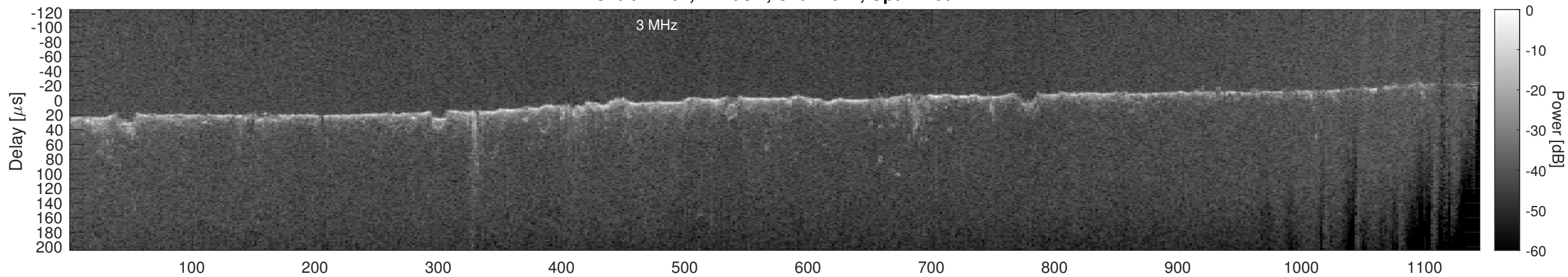
Orbit 11167, Cluttergram
