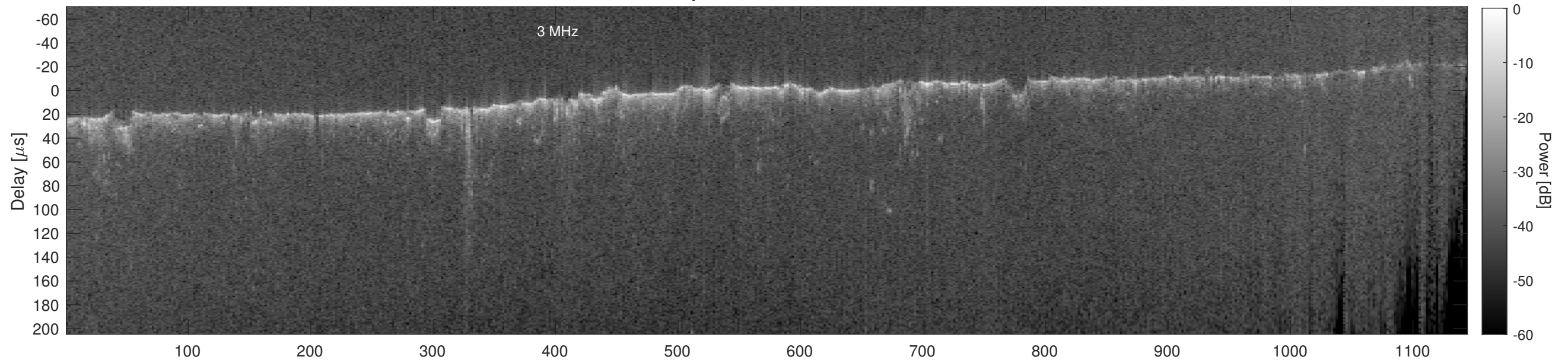
Orbit 11167, Cluttergram
