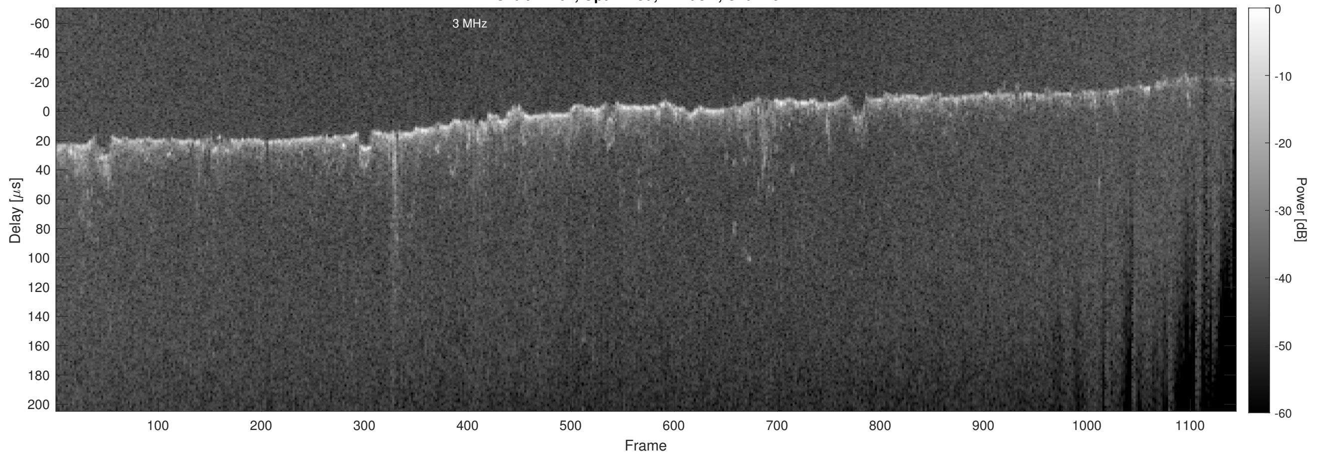
Orbit 11167, Optimized, Window, Channel 2
