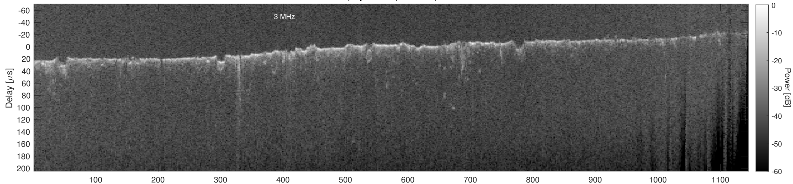
Orbit 11167, Cluttergram
