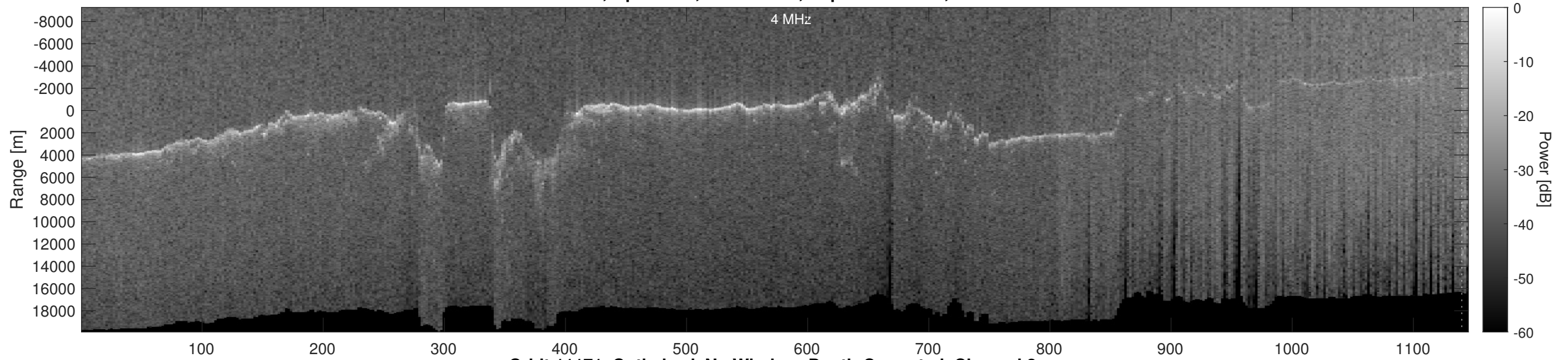
Orbit 11171, Optimized, No Window, Depth-Corrected, Channel 2
