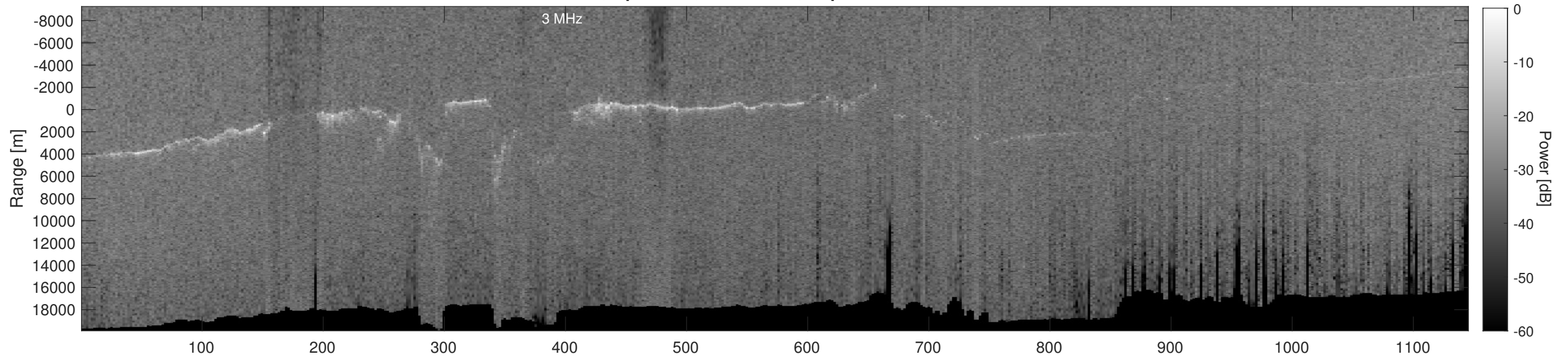
Orbit 11171, Depth-Corrected Cluttergram
