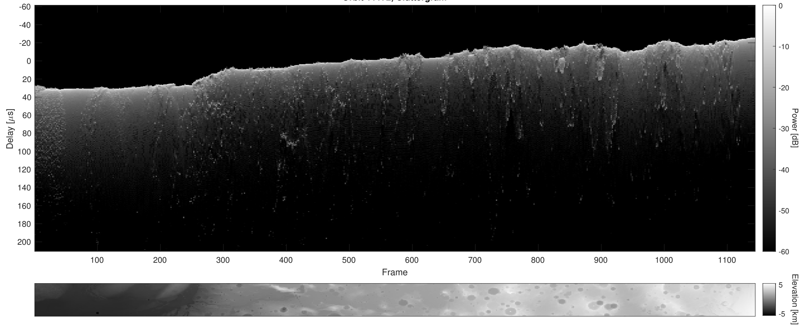
Orbit 11172, Cluttergram
