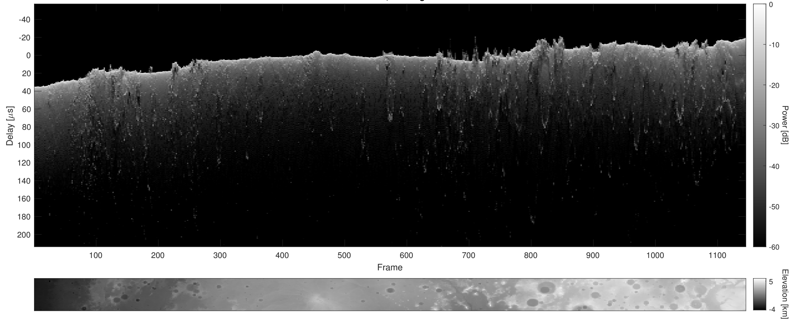
Orbit 11173, Cluttergram
