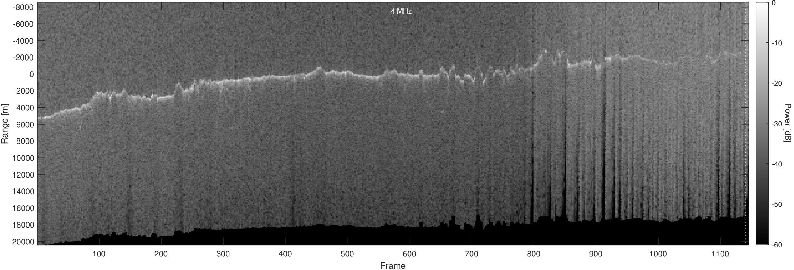
Orbit 11173, Optimized, No Window, Depth-Corrected, Channel 2
