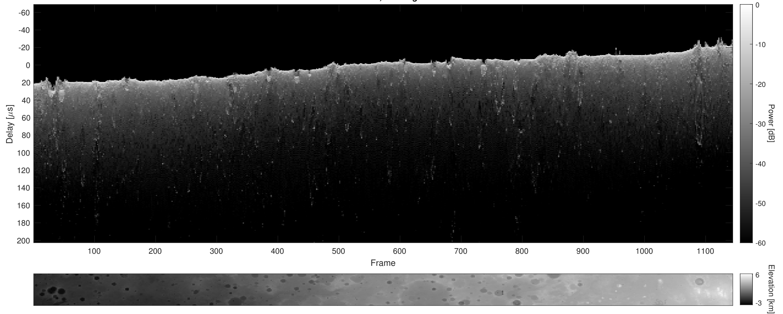
Orbit 11174, Cluttergram
