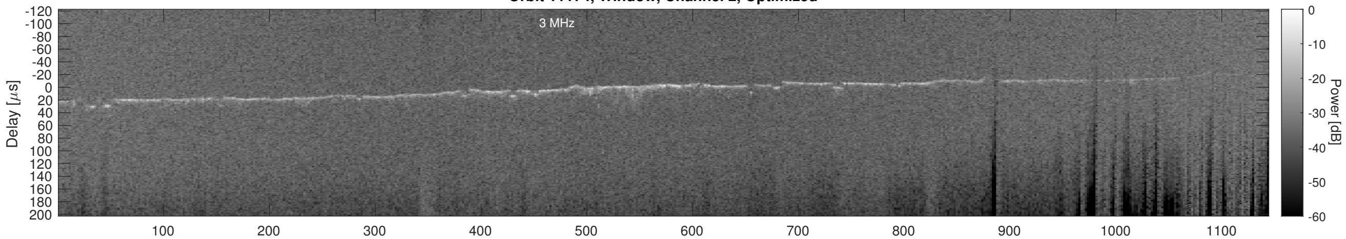
Orbit 11174, Cluttergram
