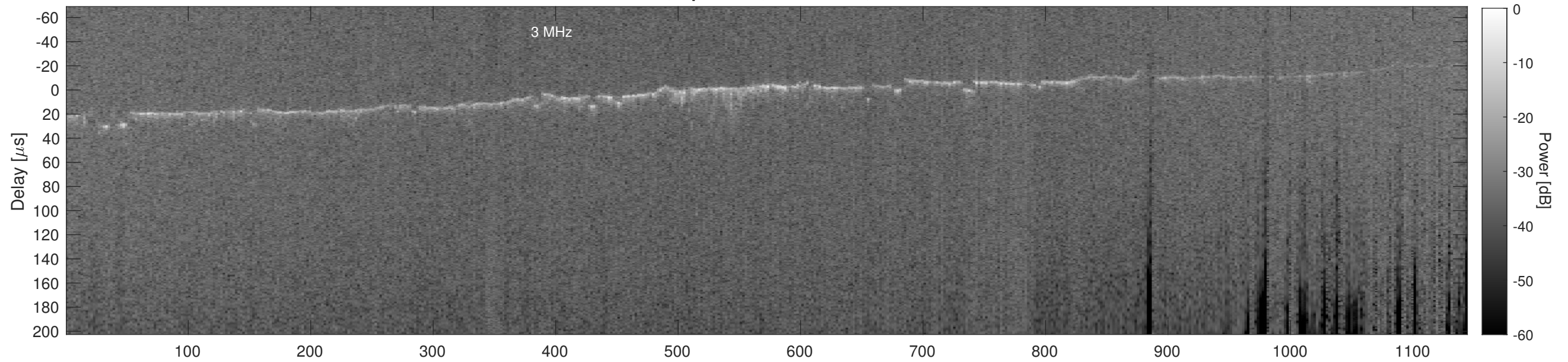
Orbit 11174, Cluttergram
