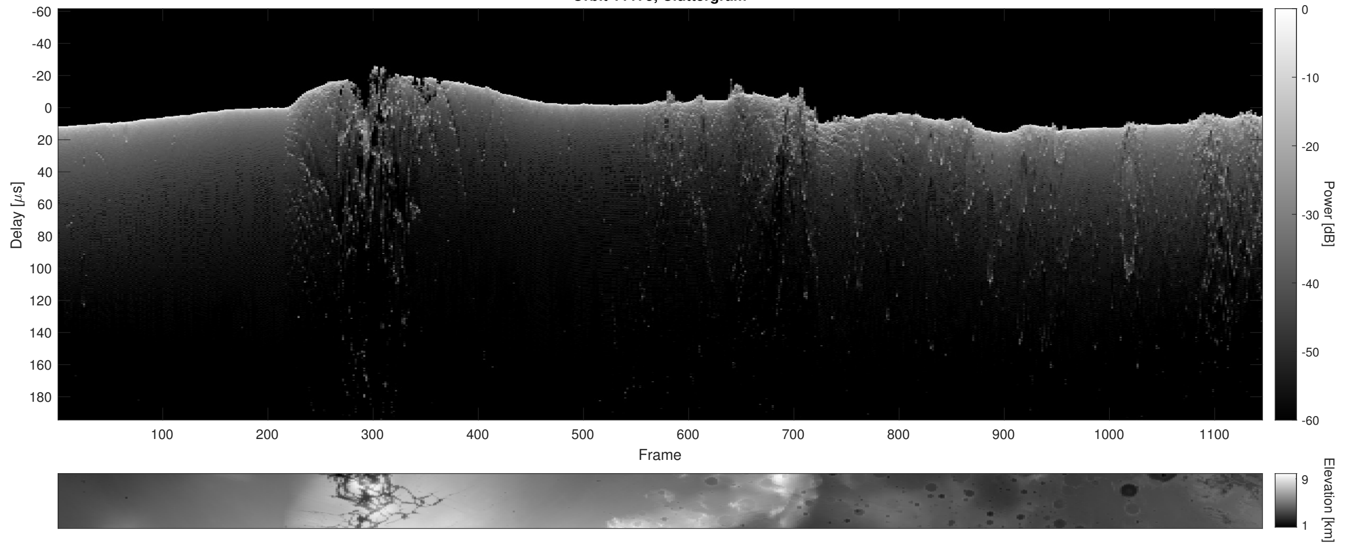
Orbit 11175, Cluttergram
