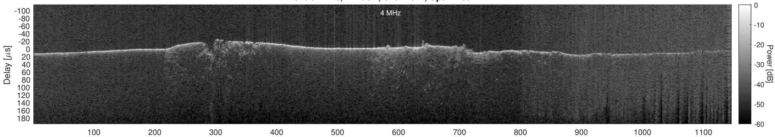
Orbit 11175, Cluttergram
