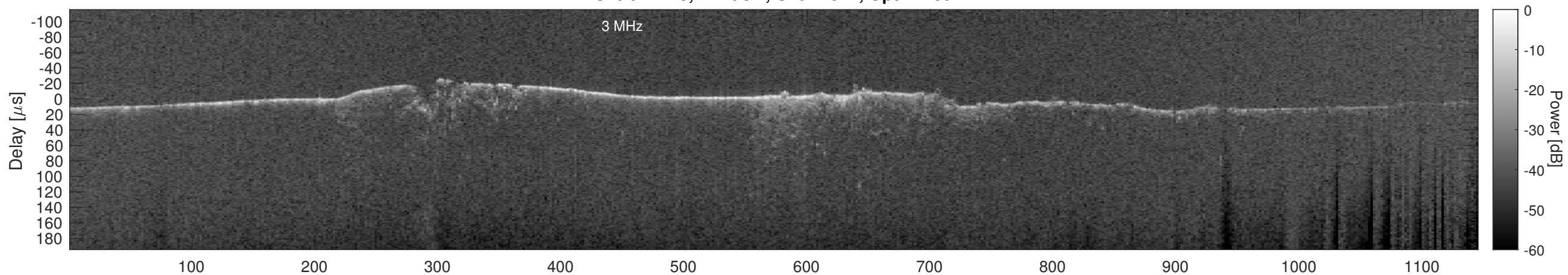
Orbit 11175, Cluttergram
