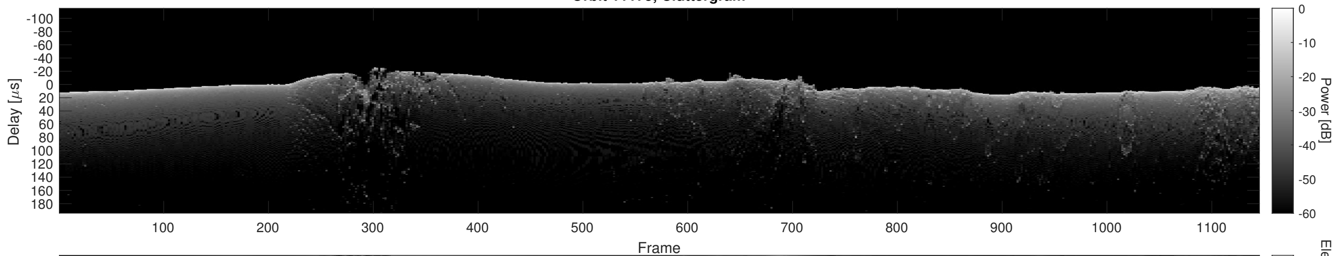
Orbit 11175, Cluttergram
