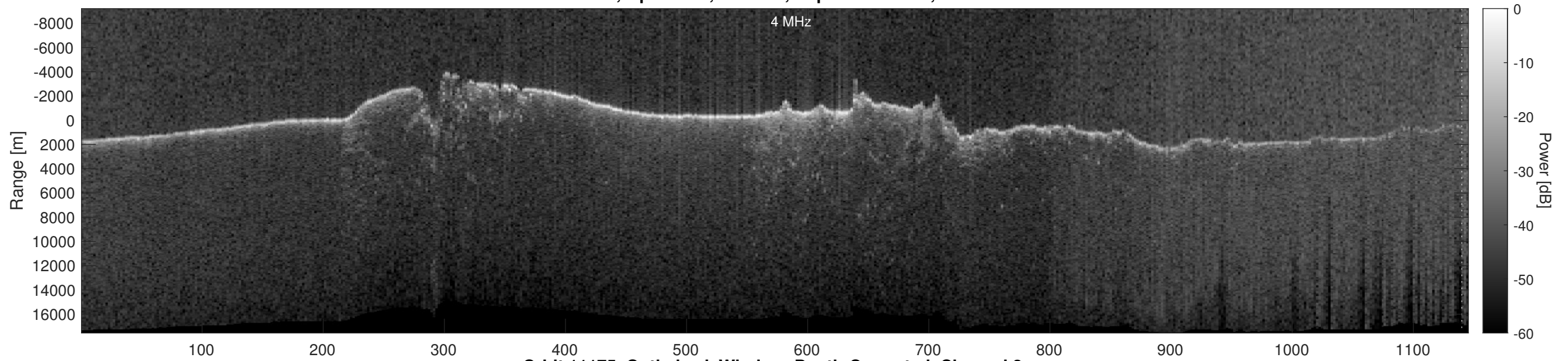
Orbit 11175, Optimized, Window, Depth-Corrected, Channel 2
