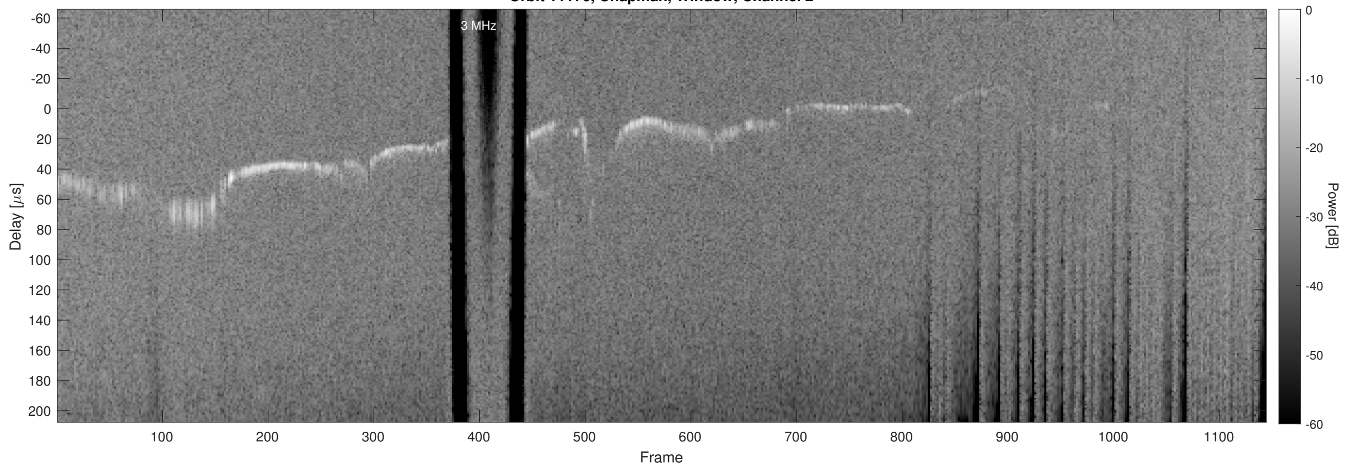
Orbit 11176, Chapman, Window, Channel 2
