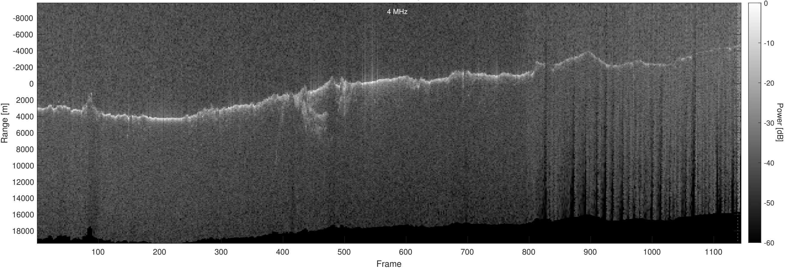
Orbit 11176, Optimized, No Window, Depth-Corrected, Channel 2
