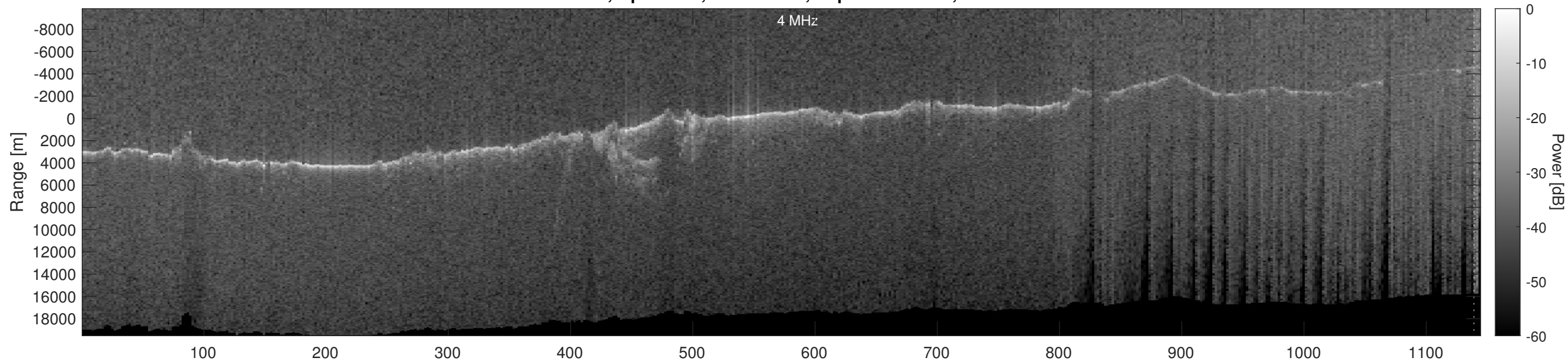
Orbit 11176, Optimized, No Window, Depth-Corrected, Channel 2
