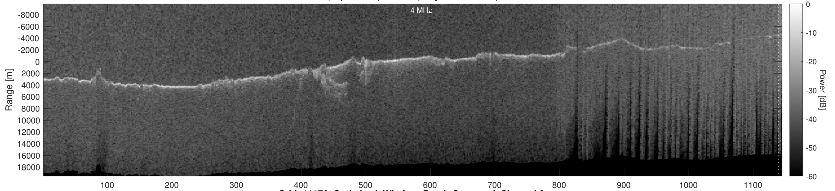
Orbit 11176, Optimized, Window, Depth-Corrected, Channel 2
