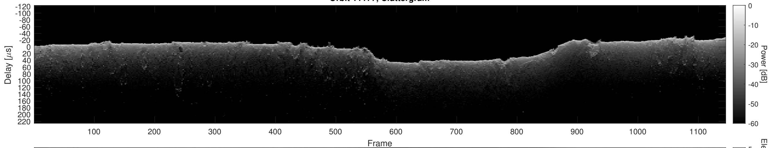
Orbit 11177, Cluttergram
