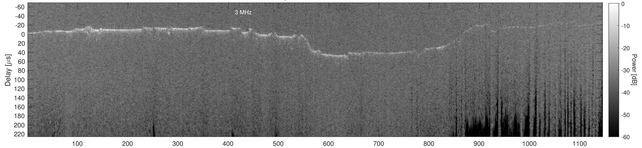
Orbit 11177, Cluttergram
