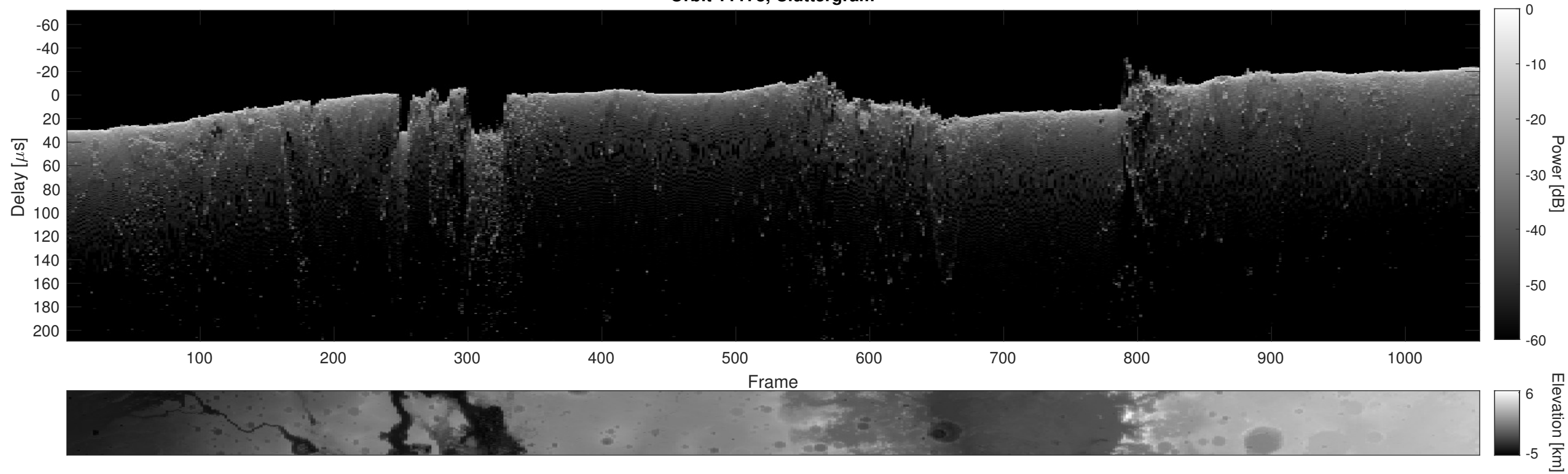
Orbit 11178, Cluttergram
