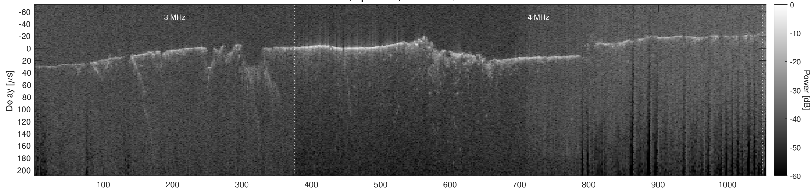
Orbit 11178, Optimized, No Window, Channel 2
