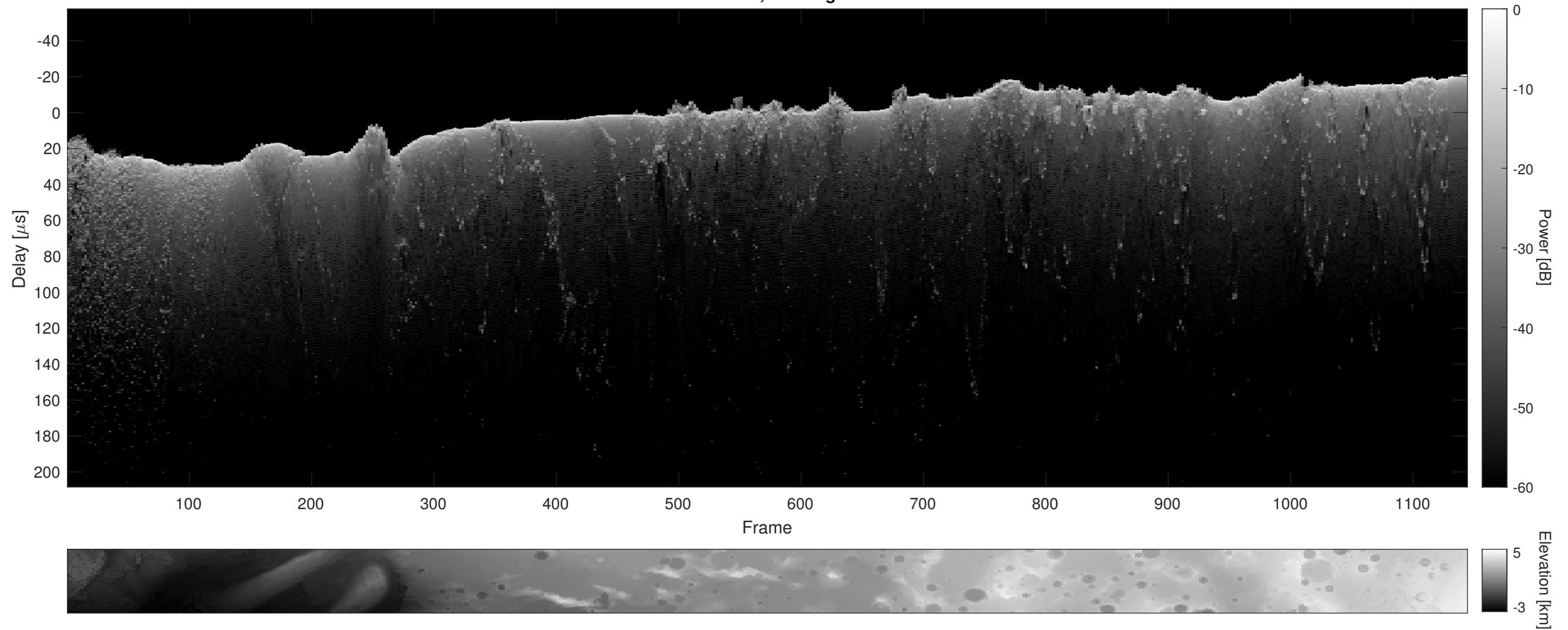
Orbit 11179, Cluttergram
