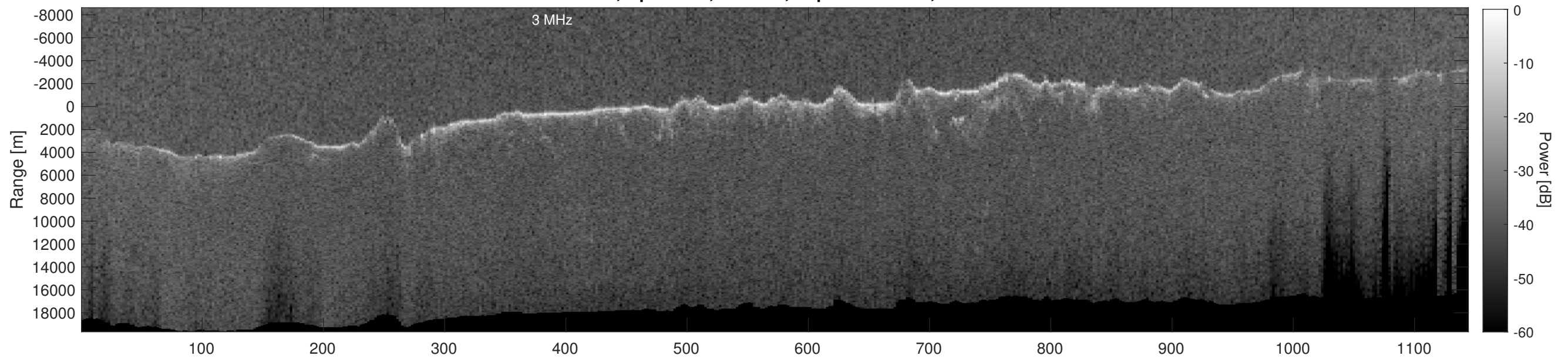
Orbit 11179, Depth-Corrected Cluttergram
