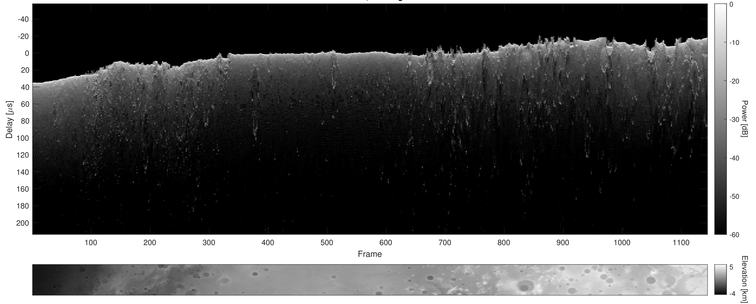
Orbit 11180, Cluttergram
