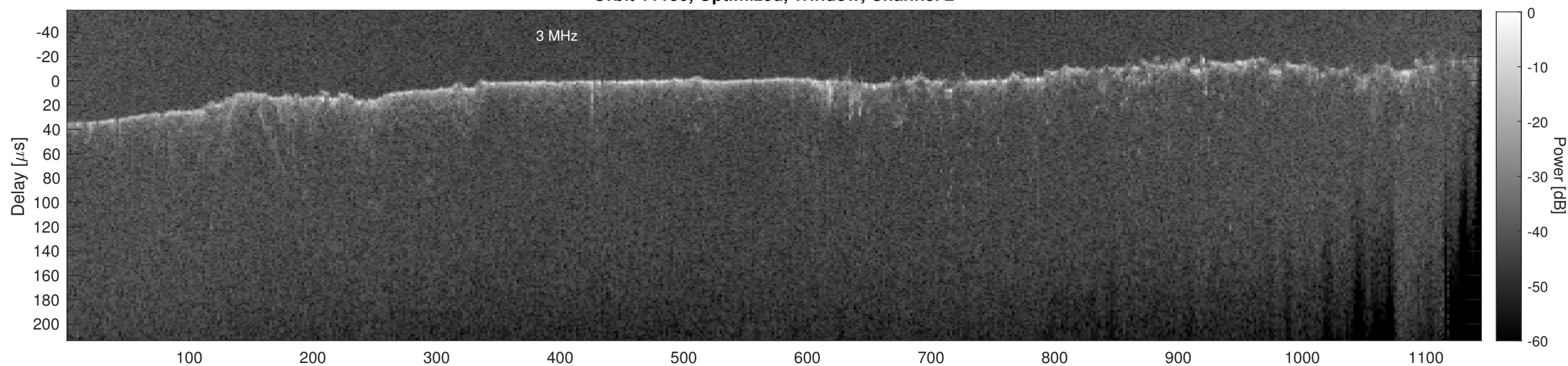
Orbit 11180, Cluttergram
