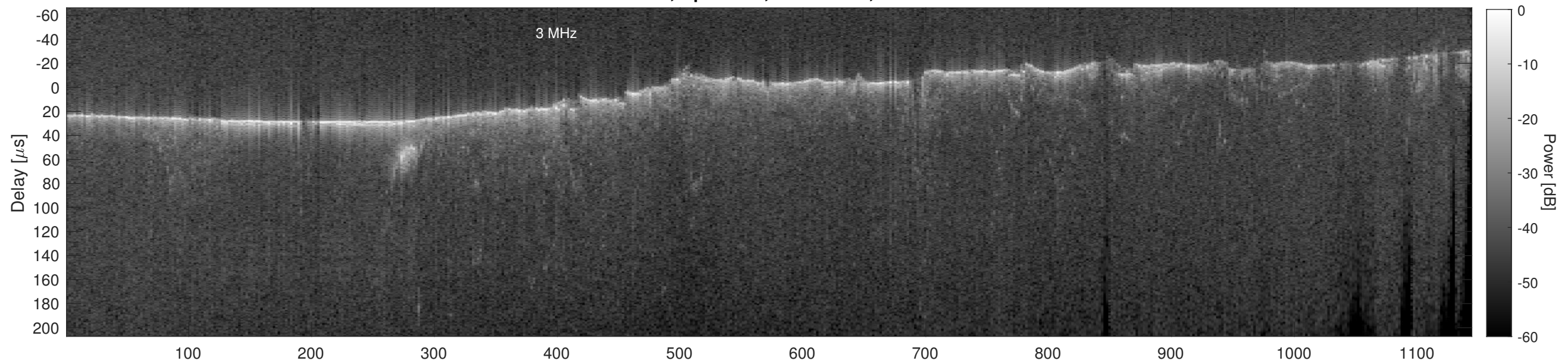
Orbit 11183, Cluttergram
