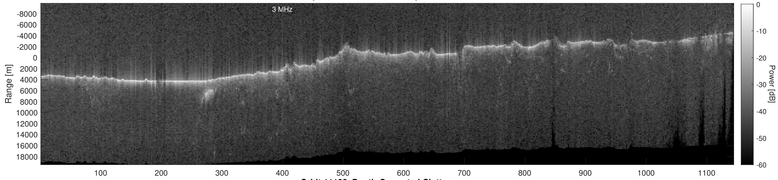
Orbit 11183, Depth-Corrected Cluttergram
