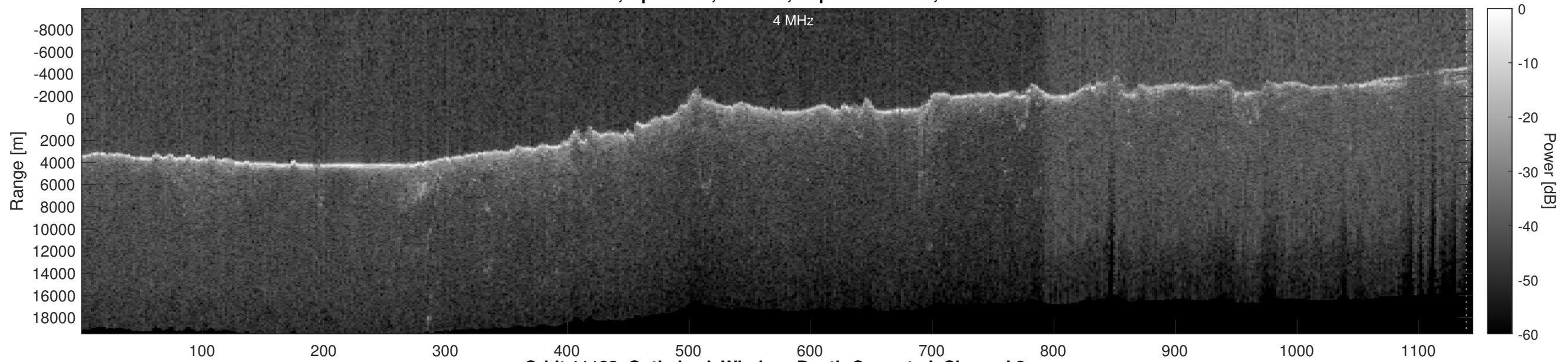
Orbit 11183, Optimized, Window, Depth-Corrected, Channel 2
