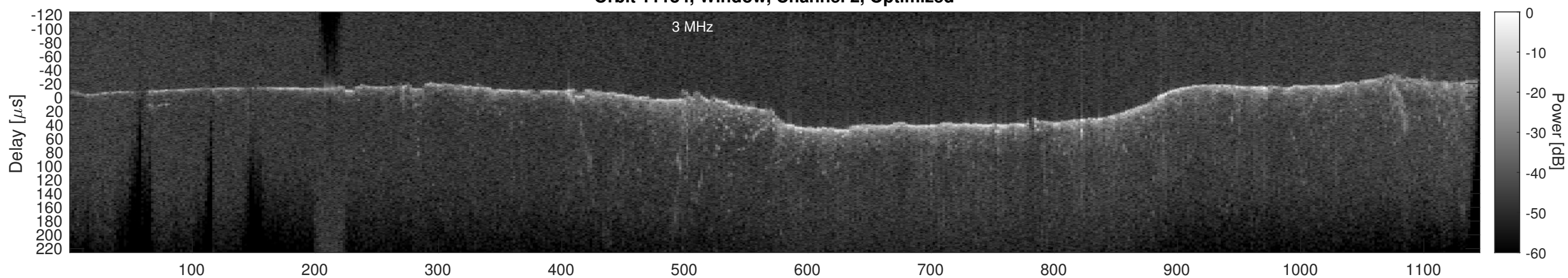
Orbit 11184, Cluttergram
