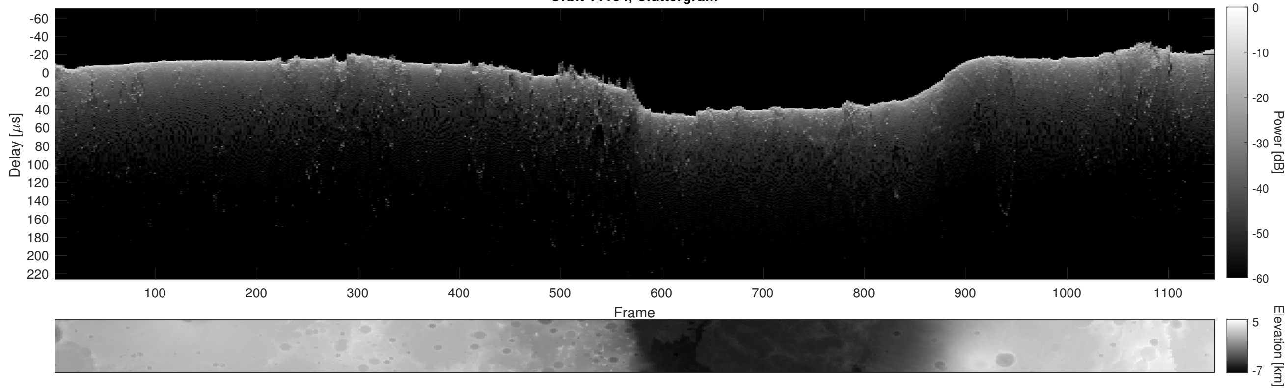
Orbit 11184, Cluttergram
