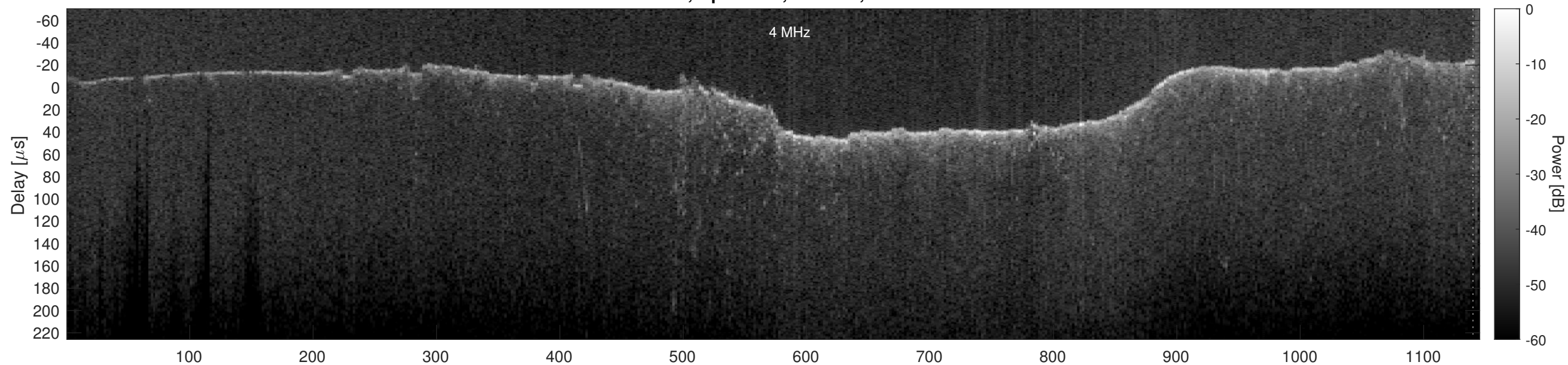
Orbit 11184, Optimized, Window, Channel 2
