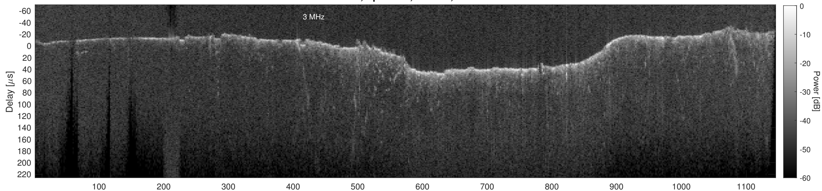
Orbit 11184, Cluttergram
