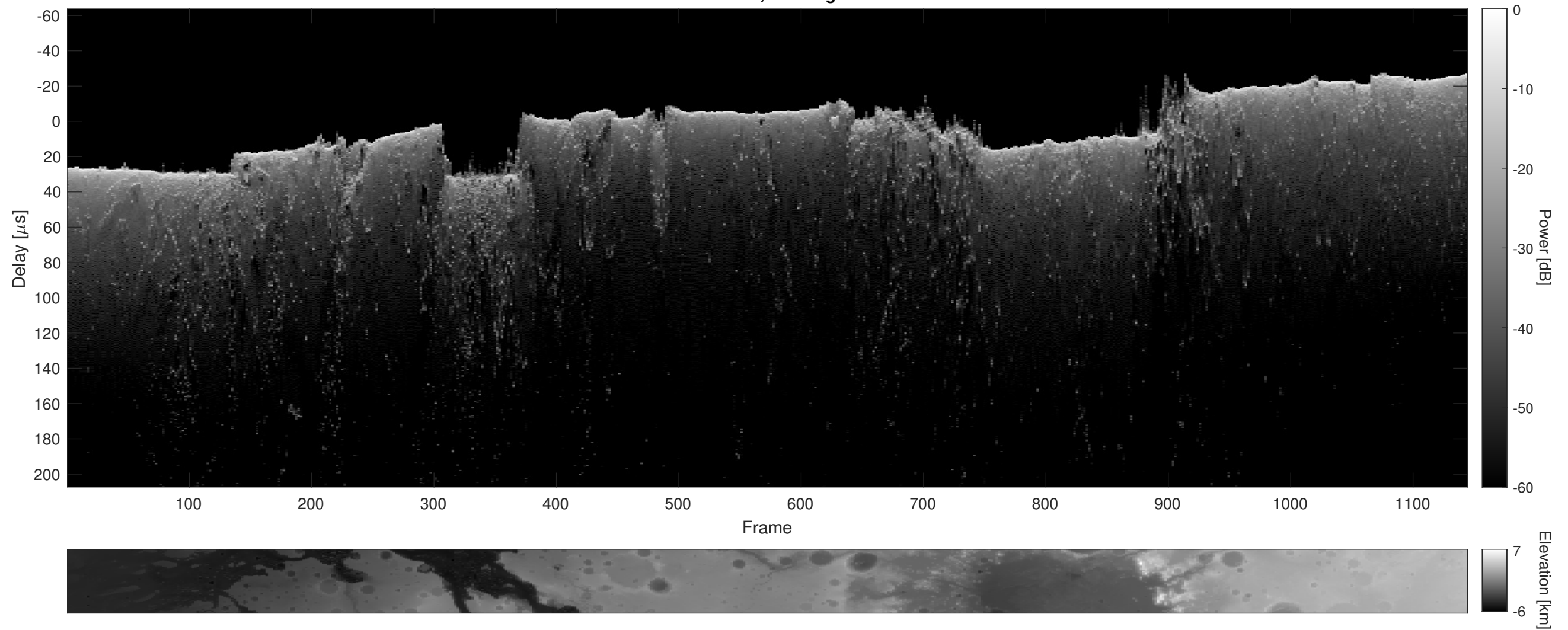
Orbit 11185, Cluttergram
